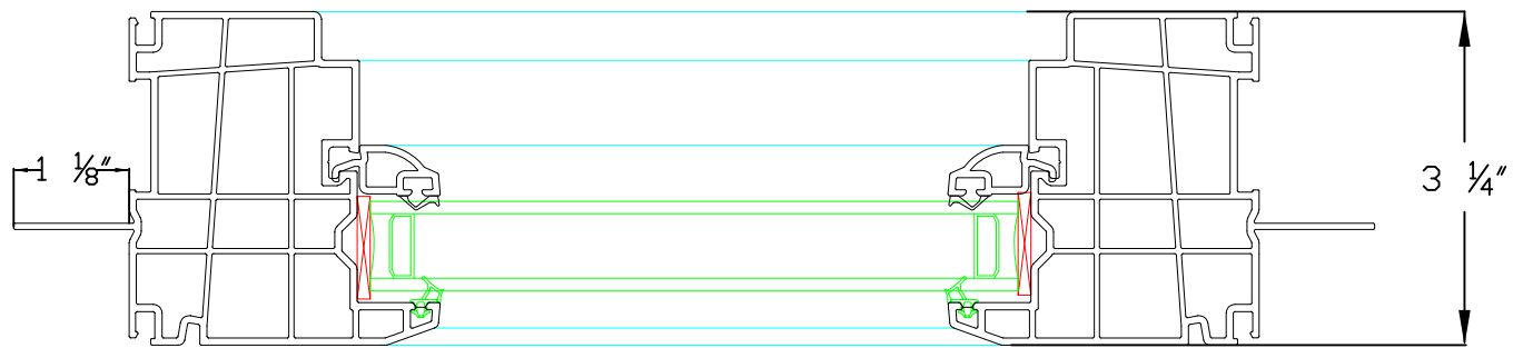
Section B-B
